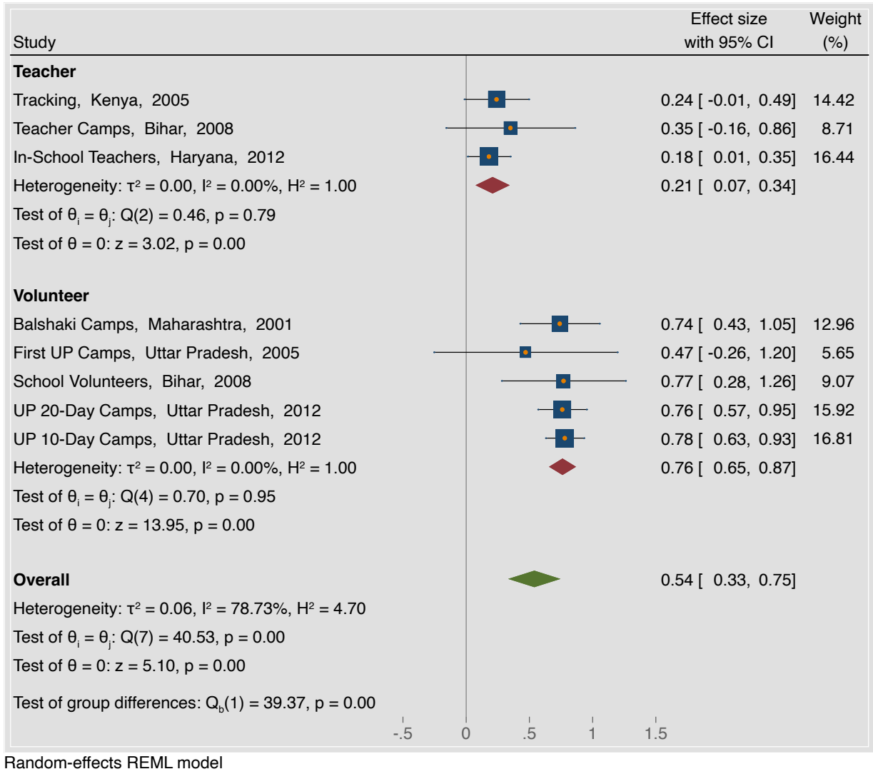
Figure 2: Frequentist Random Effects Meta-analysis of Treatment-on-Treated effects
