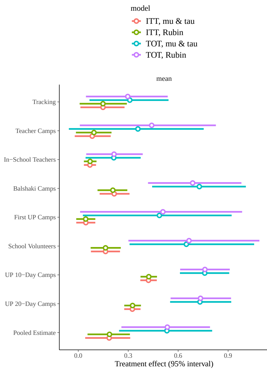
Figure A7: Rubin (1981) model vs joint "mu and tau" model
