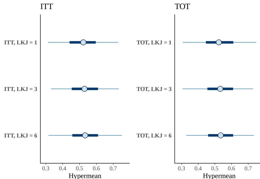
Figure A9: Mu-tau model with different LKJ priors
